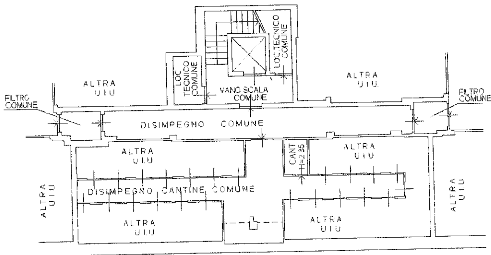
PIANO INTERRATO
